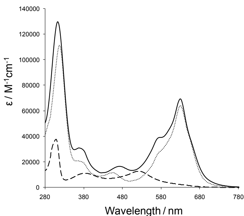
Figure 4. UV-visible spectra of 9 (dotted line), 12 (dashed line) and 1b (solid line) in dichloromethane.
