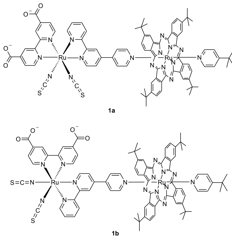
Figure 2: The ruthenium dyads, 1a and 1b that incorporate bis(bipyridyl)ruthenium(II) and ruthenium phthalocyanine chromophores.
