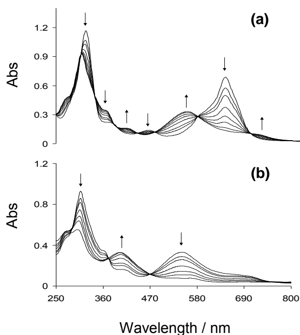
Figure 6. UV-Vis spectra recorded during the oxidative electrolyses of 9 in dichloromethane (0.1 M [n\text{-Bu}_4\text{N}][\text{PF}_6] ). (a) first oxidation process at 0.15 V. (b) second oxidation process at 0.82 V.
