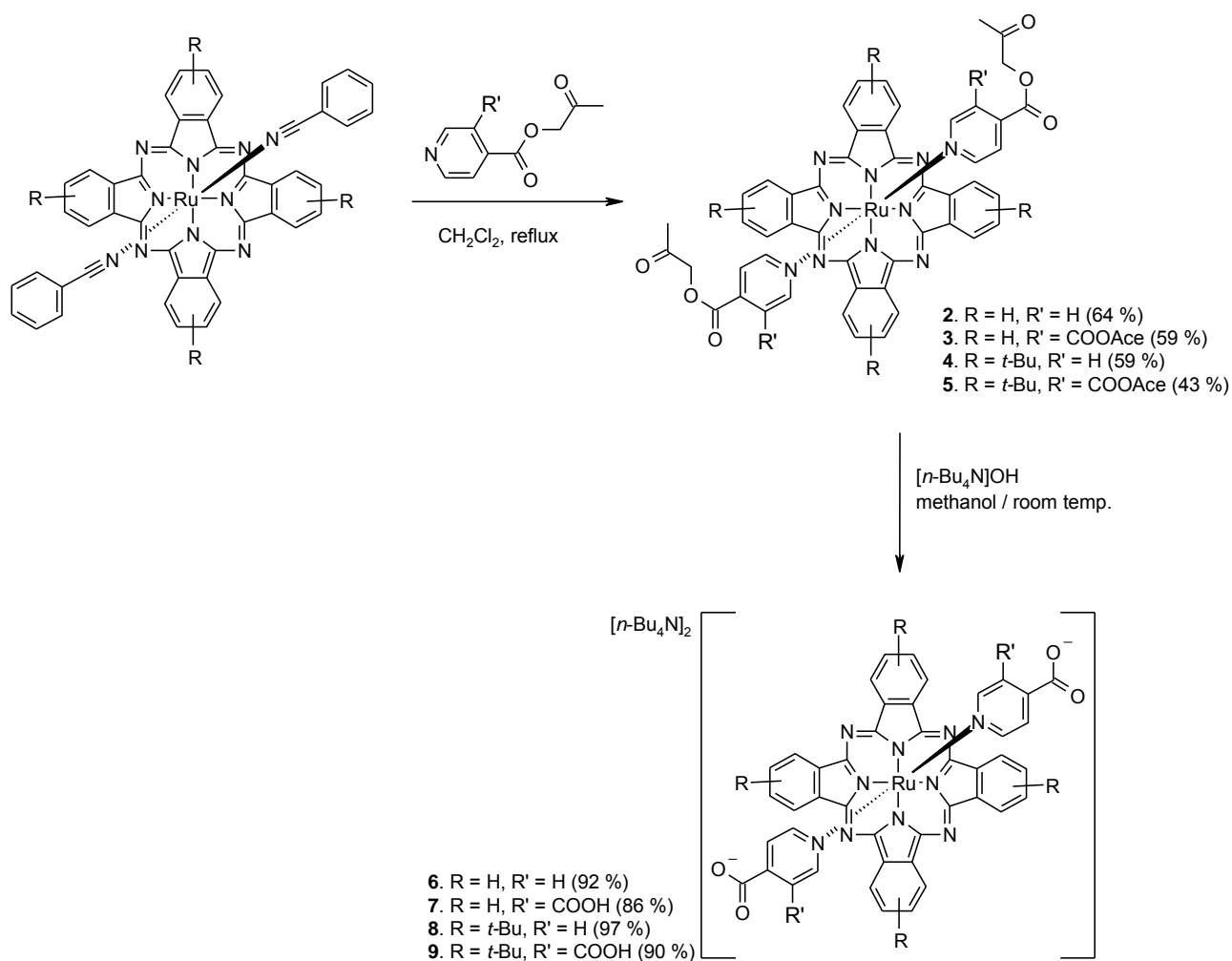
Scheme 1. Synthesis of the ruthenium phthalocyanine sensitizing complexes.
