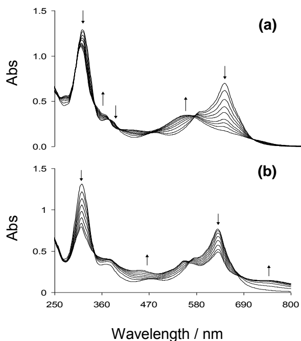
Figure 8. UV-Vis spectra recorded during the oxidative electrolyses of 1b in dichloromethane (0.1 M [n\text{-Bu}_4\text{N}][\text{PF}_6] ): (a) first oxidation process at 0.26 V; (b) second reduction process at -1.95 V.
