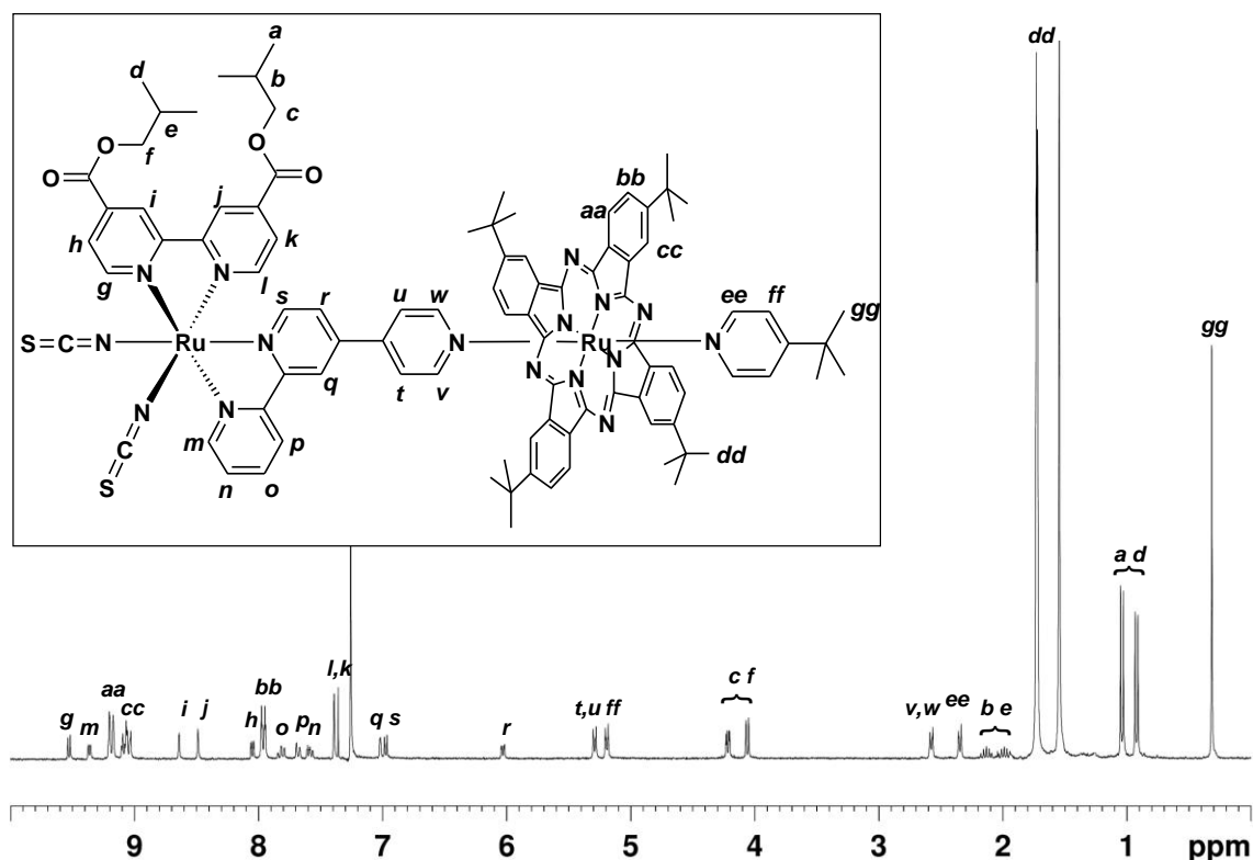
Figure 3. The ^1\text{H} NMR spectrum of 13b in \text{CDCl}_3 with peak assignments.
