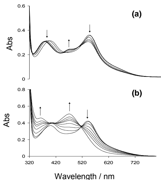
Figure 7. UV-Vis spectra recorded during the reduction (a) and first oxidation (b) of 12 in dichloromethane/DMF (0.1 M/0.2 [ n -Bu 4 N][PF 6 ] for the oxidation/reduction) using a Pt electrode.
