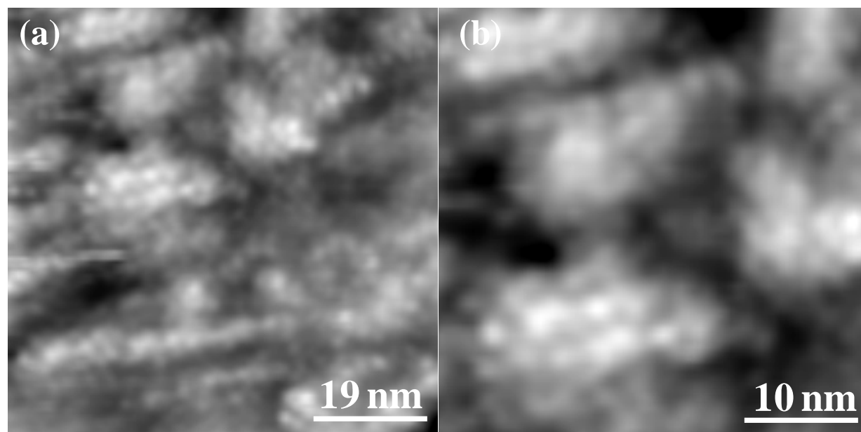
Figure 4. STM images of a thin film of 4 on Au(111). Panel (b) shows a magnified image of the central region of the image shown in (a).
