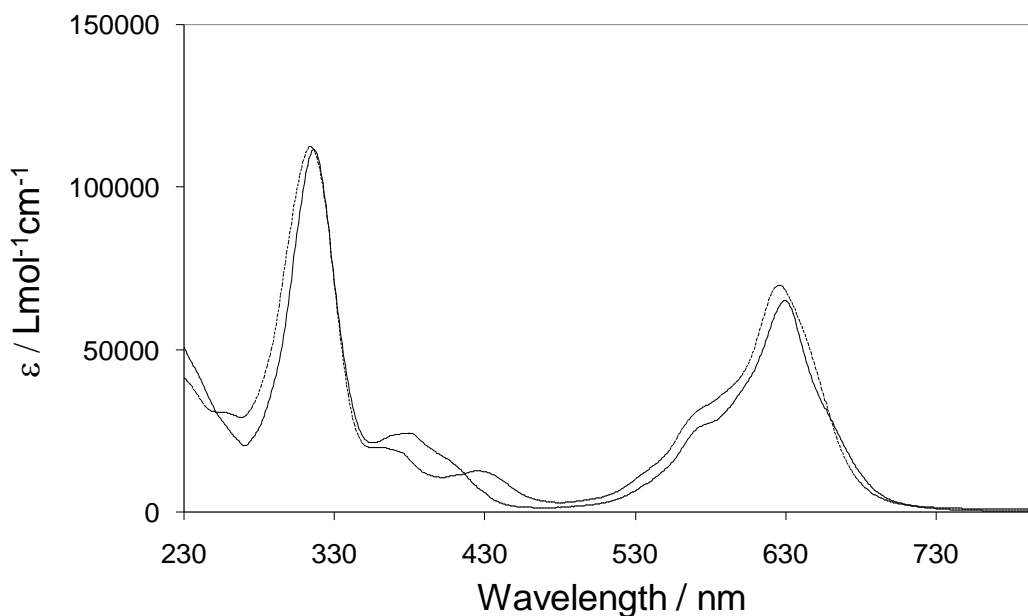
Figure 2. UV-visible spectra of 1 and 2 in dichloromethane solution.
