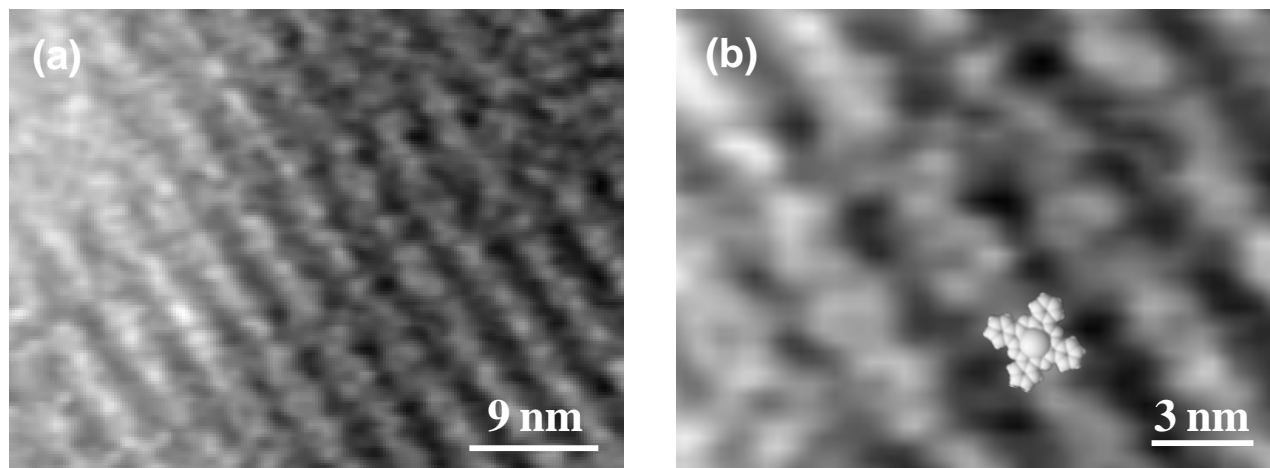
Figure 3. STM images of a thin film of 1 on a Au(111) surface. Panel (b) shows a magnified image and contains a model of the PcRu unit overlaid on the STM image. Image 2(b) is contrast-enhanced by applying a correlation averaging procedure and a low-pass filter.
