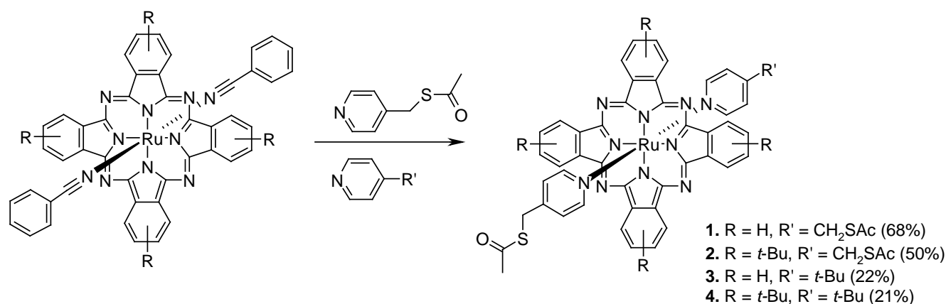
Scheme 1. Synthesis of the monomeric complexes 1–4 .
