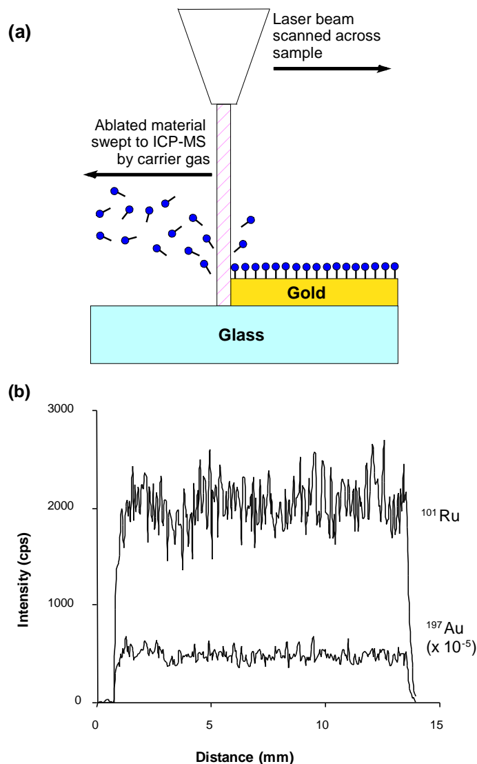
Figure 5. a) Diagram showing the laser ablation of ruthenium phthalocyanine molecules together with the underlying gold layer. (b) LA-ICP-MS signals of ^{101}\text{Ru} and ^{197}\text{Au} generated from a single scan of a thin film of the ruthenium phthalocyanine complex on gold.
