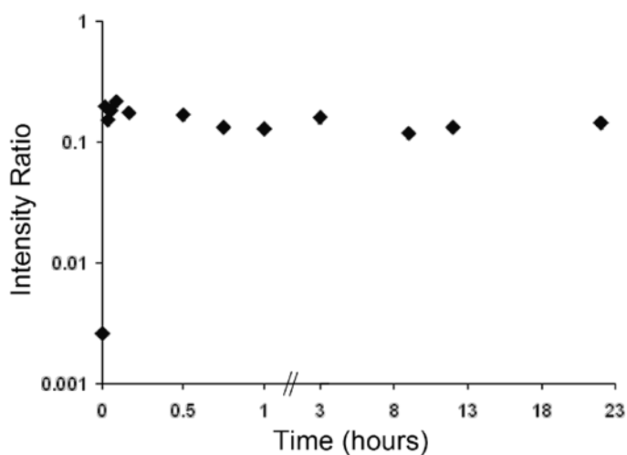
Figure 6. Intensity ratio ( ^{101}\text{Ru}: ^{97}\text{Mo} ) vs immersion time of gold surfaces in a [(t\text{-Bu})_4\text{Pc}]\text{Ru}(4\text{-pyCH}_2\text{SAc})_2 / \text{TBAOH} solution.
